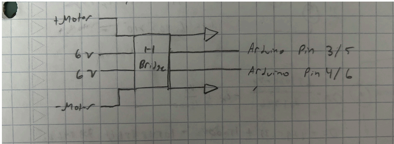
Figure B.3: Circuitry for the H-Bridges. Arduino pins 3 and 4 refer to the left motor and Arduino pins 5 and 6 refer to the right motor.
